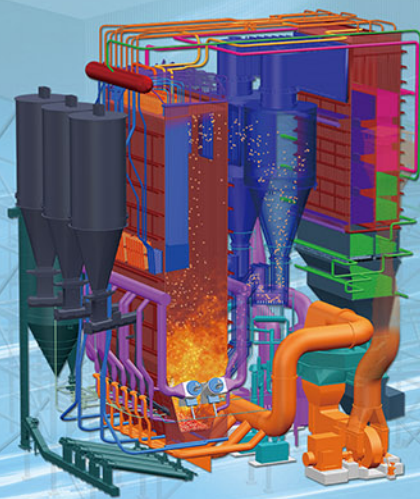
●循環流體化床鍋爐 Circulating Fluidized Bed (CFB) Boiler
